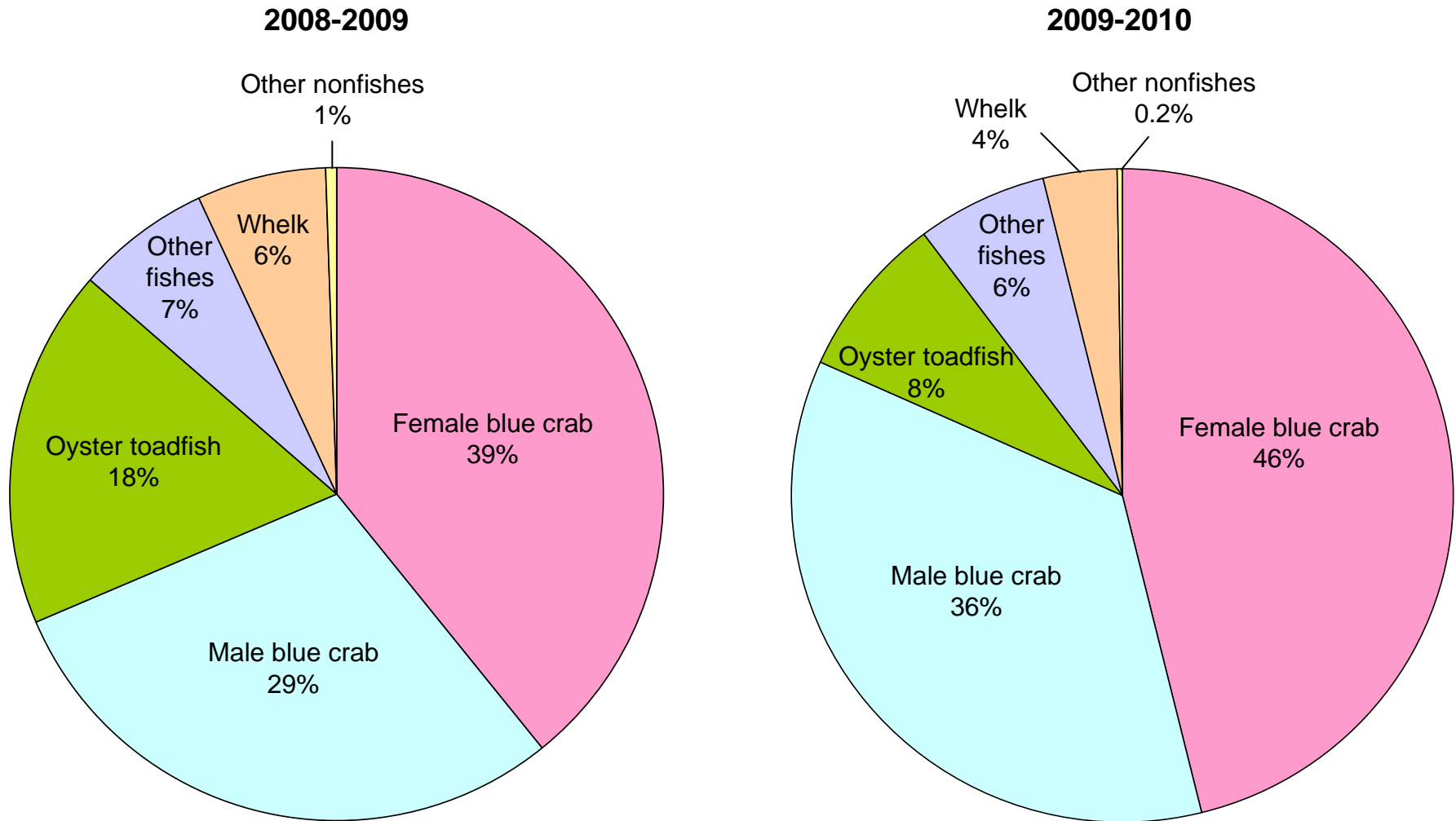
Figure 2. Percent-of-catch data from the 2008-2009 and 2009-2010 seasons of the derelict crab pot removal project.
